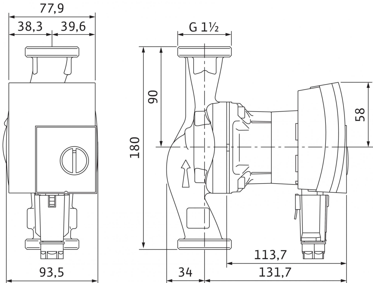
Dimension drawing
